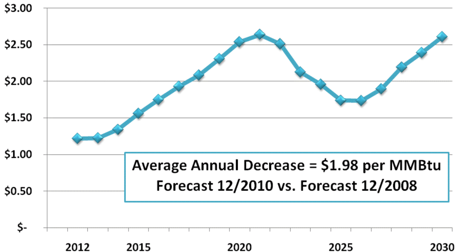
Decrease in EIA Natural Gas Price Projections AEO2011 vs. Updated AEO2009 ($/MMBtu) @ Henry Hub
